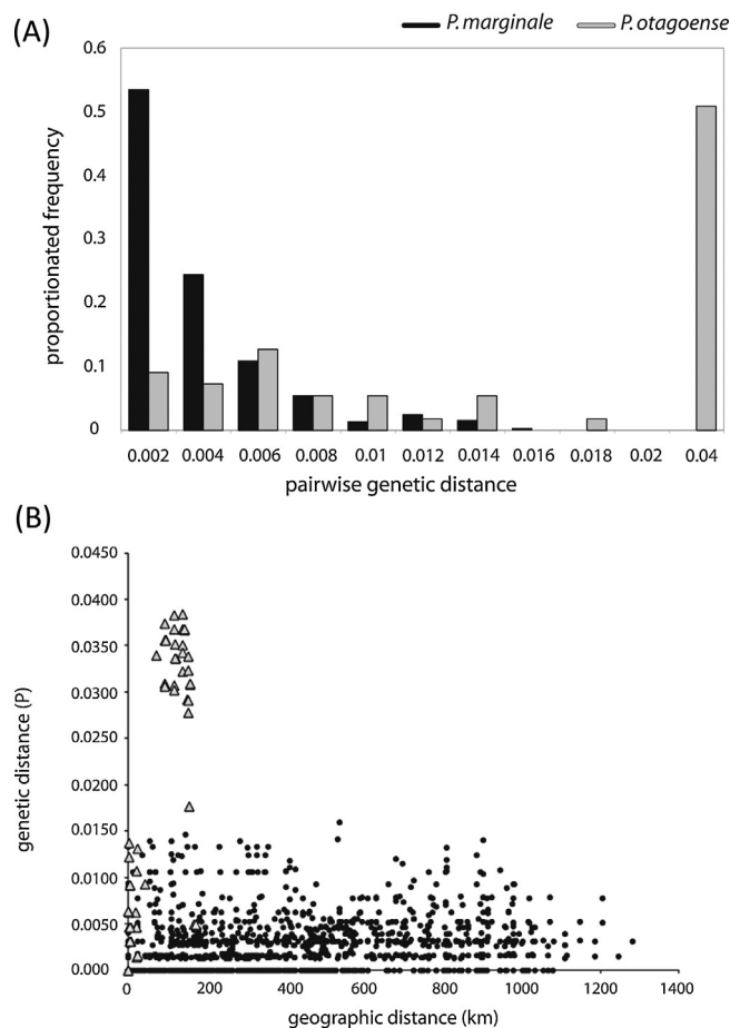
Fig. 3. Mismatch distributions calculated for P. marginale (black) and P. otagoense (grey) from COI mtDNA illustrating the differences in genetic divergence within the two species. (A) Frequency distribution plot based on proportionated frequencies and pairwise genetic distances highlighting the difference in frequency distribution in the two species, with P. marginale mostly exhibiting low genetic distances (up to 1.5%) and P. otagoense showing the highest frequency at approximately 4% pairwise genetic distance. (B) Distribution plot based on genetic and geographic distances of individuals of the two species, depicting the high genetic divergence coupled with a narrow geographic range in P. otagoense (grey triangles) and the opposite – low genetic distance within a wider geographic distribution – in P. marginale (black dots).
