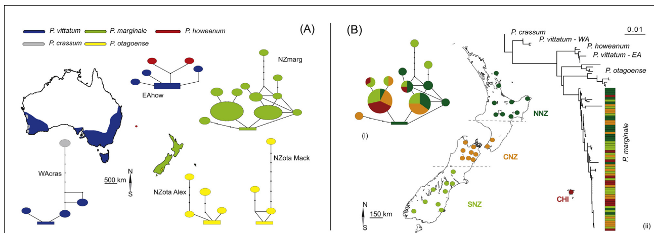
Fig. 2. Distribution of mtDNA COI diversity among Phaulacridium grasshoppers in Australia and New Zealand with haplotype networks for each taxon. (A) Australian and New Zealand region with distribution of Phaulacridium taxa, with matching colored circles in corresponding haplotype networks (NZmarg = New Zealand P. marginale , NZota Alex = New Zealand P. otagoense from Alexandra area, NZota Mack = New Zealand P. otagoense from Mackenzie area, EAhow = P. vittatum eastern Australia and P. howeanum , WAcras = P. vittatum western Australia and P. crassum ). (B) Map of New Zealand showing the four main sampling areas (three in mainland New Zealand, the fourth being the Chatham Islands) of P. marginale with sampling locations (colored circles); inset (i) shows haplotype network for P. marginale , with colors corresponding to sampling areas and depicting the frequency of the different areas within one haplotype; inset (ii) shows a neighbour-joining tree representing all sampled taxa, with colored labels of P. marginale representing haplotypes according to sampling areas and colored circles in Fig. 2B(i).
