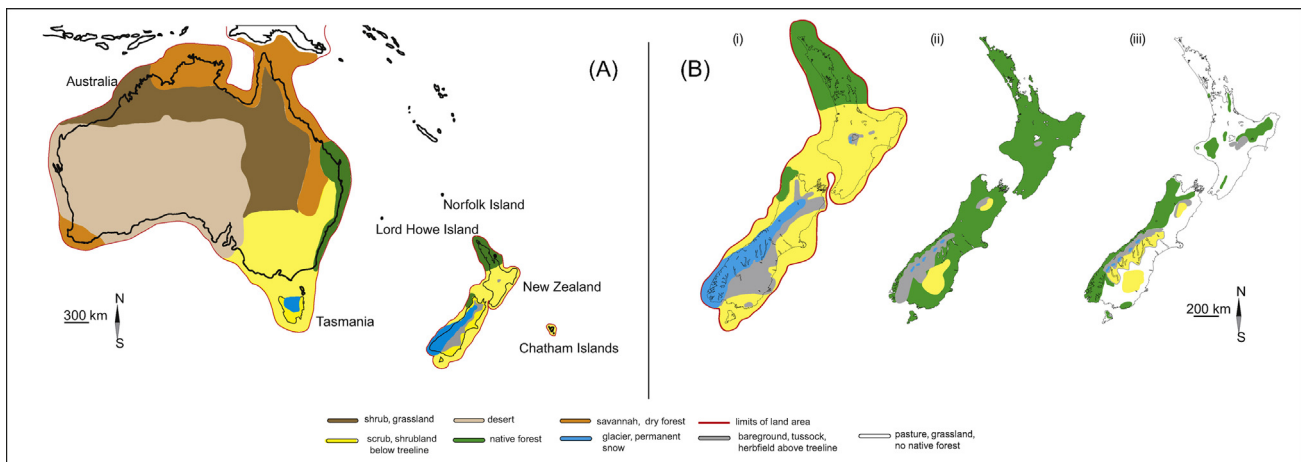
Fig. 1. Vegetation habitat zones in Australia and New Zealand; (A) Last glacial maximum (LGM), modified from Hope et al. (2004) and Alloway et al. (2007). (B) Approximate distribution of vegetation zones in New Zealand at (i) LGM, (ii) pre-human, (iii) modern (post human settlement) New Zealand (modified from Alloway et al., 2007).
