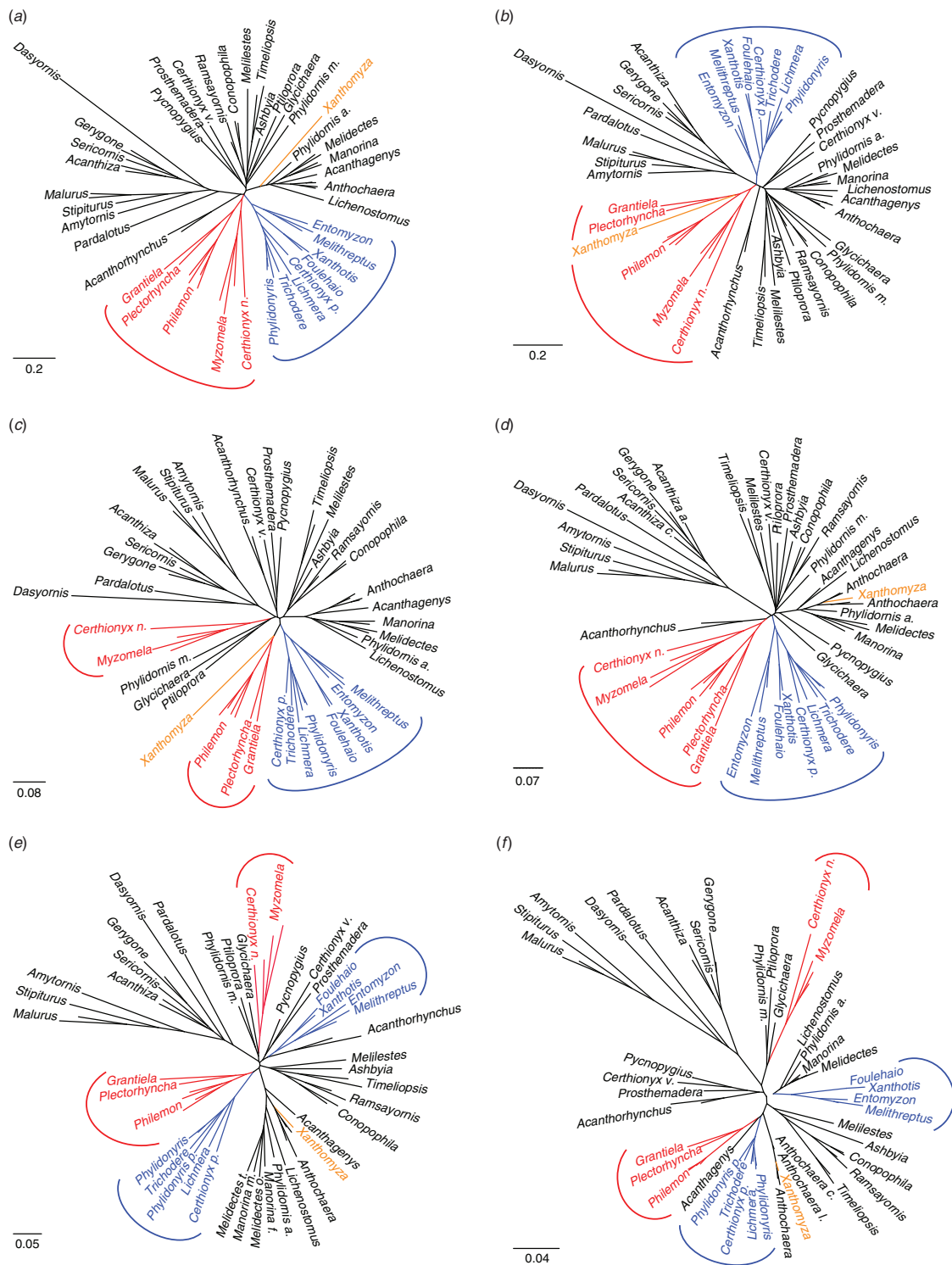
Fig. 2. Phylogenies for Meliphagidae and its relatives based on maximum likelihood analyses of identically sampled 61-taxon two-locus matrices. (a) tree based on ND2 and cytB sequences; (b) tree based on ND2 and 12S sequences; (c) tree based on ND2 and Fib5 sequences; (d) tree based on cytB and 12S sequences; (e) tree based on cytB and Fib5 sequences; (f) tree based on 12S and Fib5 sequences. For clarity, genus names are given when the genus is represented by a single species or where all (or most) sampled members form a clade; where a genus is not monophyletic the first letter of the species epithet is given to distinguish it from other members of the genus (see Table S1 for list of included species). The two reference clades (and their relatives), as described in the text, are highlighted in red ( Myzomela plus Certhionyx niger ) and blue ( Foulehaio – Xanthotis ) with Xanthomyza highlighted in orange to illustrate positional instability.
