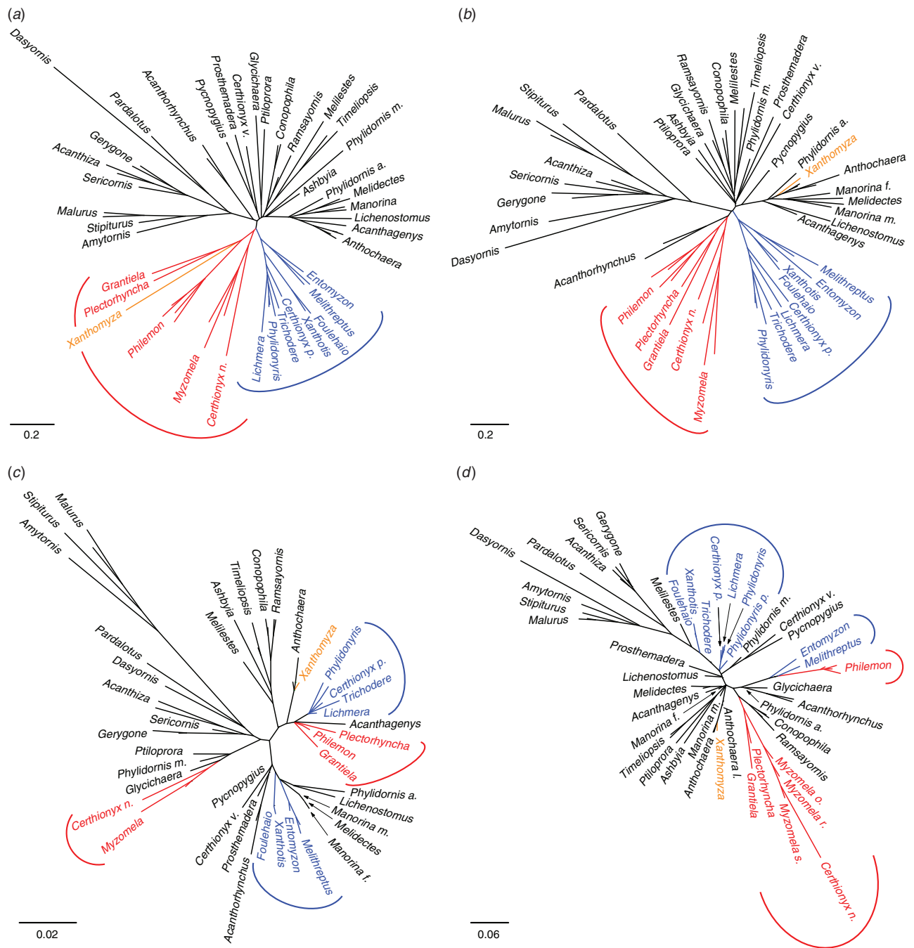
Fig. 1. Phylogenies for Meliphagidae and its relatives based on maximum likelihood analyses of identically sampled 61-taxon single-locus matrices. (a) tree based on ND2 sequences; (b) tree based on cytB sequences; (c) tree based on Fib5 sequences; (d) tree based on 12S sequences. For clarity, genus names are given when the genus is represented by a single species or if all (or most) sampled members form a clade; where a genus is not monophyletic the first letter of the species epithet is given to distinguish it from other members of the genus (see Table S1 for list of included species). The two reference clades (and their relatives), as described in the text, are highlighted in red ( Myzomela plus Certhionyx niger ) and blue ( Foulehaio – Xanthotis ) with Xanthomyza highlighted in orange to illustrate positional instability.
