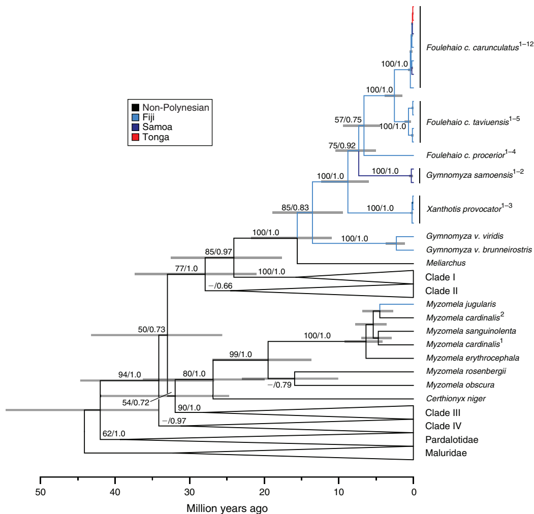
Fig. 3. The maximum clade credibility tree from BEAST analyses of ND2 sequences for Meliphagidae and relatives. Branch lengths are proportional to time with grey bars indicating 95% highest posterior densities on node ages. Genus, species, and, where appropriate, subspecies epithets are given for groups with Fijian representatives; resolution for clades not represented in Fiji is collapsed. Clade I contains species of Certhionyx , Lichmera , Phylidonyris and Trichodere ; Clade II contains Entomyzon , Lichenostomus and Melithreptus ; Clade III contains Philemon and Xanthotis ; Clade IV includes representatives of 22 genera including Certhionyx , Lichenostomus and Phylidonyris (see Table S1 for list of included species; full tree available on request). For groups with Fijian representatives, branches are coloured on the basis of maximum parsimony inference of ancestral character states. Support values are given for branches. The first number is the maximum likelihood bootstrap support (estimated using phyML), the second is the posterior probability; a dash indicates that the bootstrap value was below 50%. For clarity, values are omitted for relationships within subspecies of Foulehaio .
